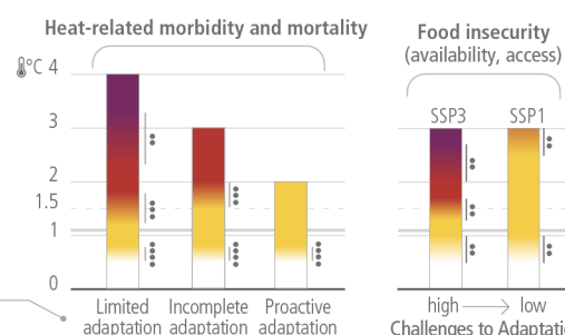
Figure SPM.4: Subset of assessed climate outcomes and associated global and regional climate risks. The burning embers result from a literature based expert elicitation. Panel (a): Left – Global surface temperature changes in °C relative to 1850–1900. These changes were obtained by combining CMIP6 model simulations with observational constraints based on past simulated warming, as well as an updated assessment of equilibrium climate sensitivity. Very likely ranges are shown for the low and high GHG emissions scenarios (SSP1-2.6 and SSP3-7.0) (Cross-Section Box 2); Right – Global Reasons for Concern (RFC), comparing AR6 (thick embers) and AR5 (thin embers) assessments. Risk transitions have generally shifted towards lower temperatures with updated scientific understanding. Diagrams are shown for each RFC, assuming low to no adaptation. Lines connect the midpoints of the transitions from moderate to high risk across AR5 and AR6. Panel (b): Selected global risks for land and ocean ecosystems, illustrating general increase of risk with global warming levels with low to no adaptation. Panel (c): Left - Global mean sea level change in centimetres, relative to 1900.
